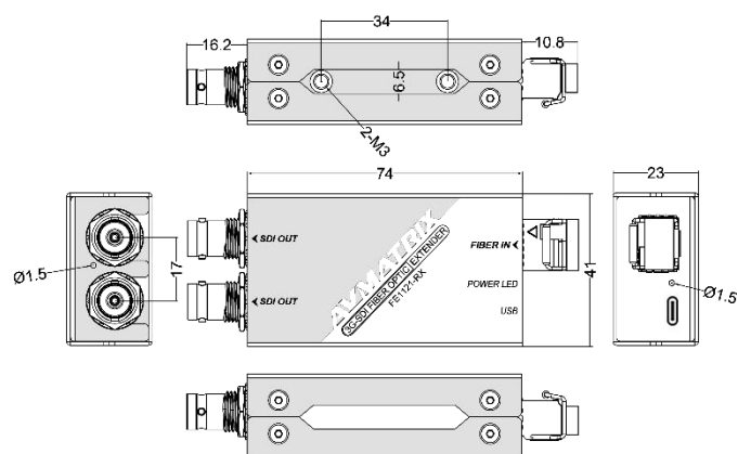
FE1121-RX(Receiver)
