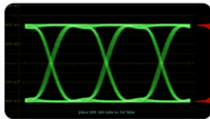
Eye Diagram
