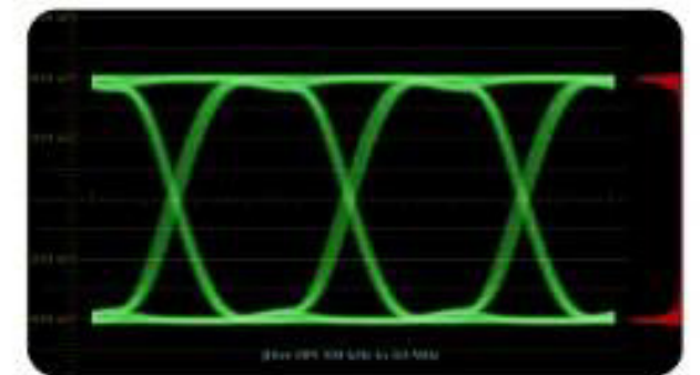
Eye Diagram
